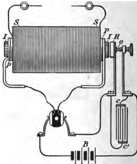
FIG. 228.—Diagram of the Essential Parts of an Induction Coil: B, chemical battery; C, C', condenser terminals; I, laminated iron core; P, primary winding; S, secondary winding; H, head of the vibrator; o, contact point of the back-stop screw.
